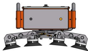
Used for curved glass ( R_{max}=800 )
