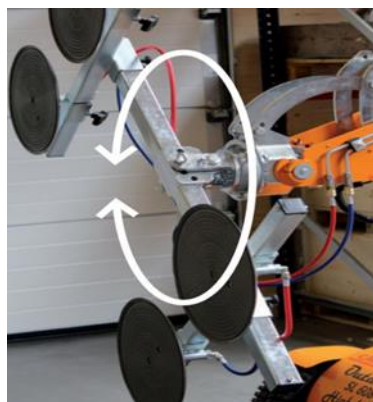
SL409 Outdoor High Lifter Rotation (electric yoke rotation)
