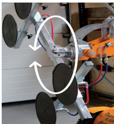
SL1009 Outdoor Rotation (electric yoke rotation)
